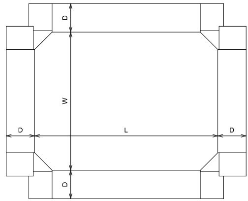
FEFCO\0400 - Folder Type Boxes\FEFCO 0459
