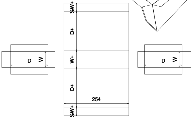
FEFCO\0600 - Rigid Type Boxes\FEFCO 0620
