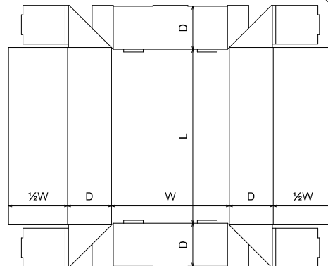
FEFCO\0400 - Folder Type Boxes\FEFCO 0437
