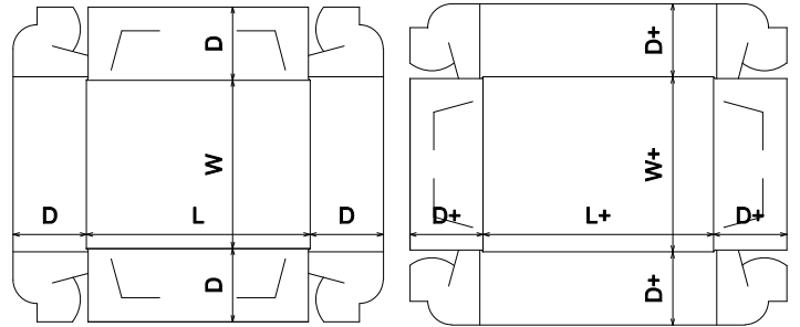
FEFCO\0300 - Telescope Type Box\FEFCO 0307
