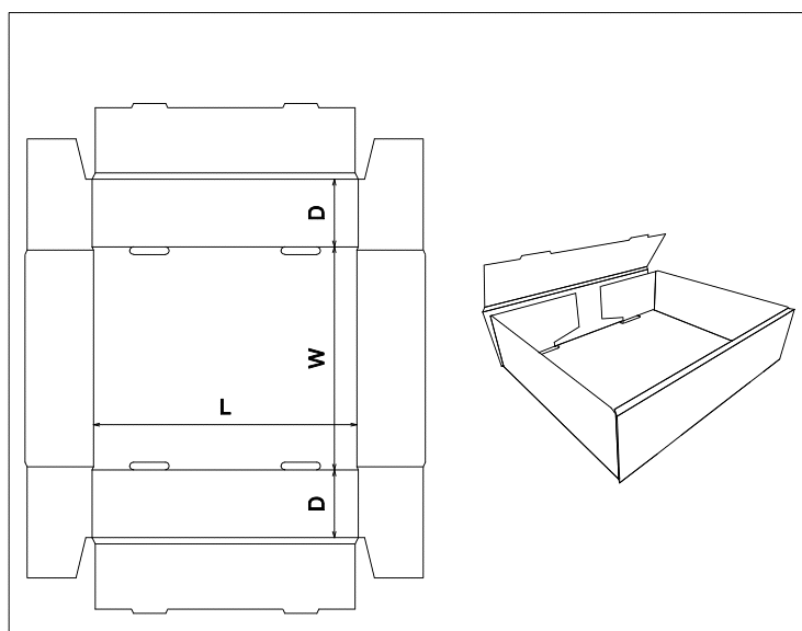
FEFCO\0400 - Folder Type Boxes\FEFCO 0425
