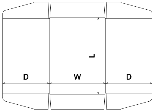
FEFCO\0400 - Folder Type Boxes\FEFCO 0460
