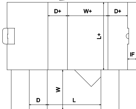
FEFCO\0400 - Folder Type Boxes\FEFCO 0473
