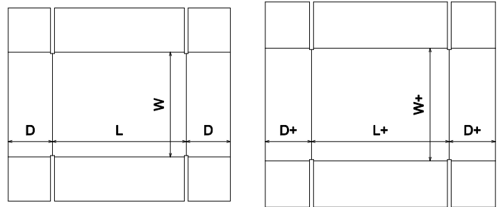
FEFCO\0300 - Telescope Type Box\FEFCO 0300
