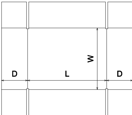
FEFCO\0400 - Folder Type Boxes\FEFCO 0452
