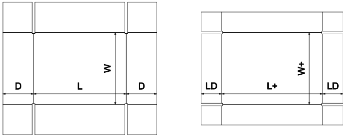
FEFCO\0300 - Telescope Type Box\FEFCO 0306
