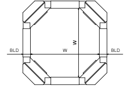
FEFCO\0300 - Telescope Type Box\FEFCO 0351
