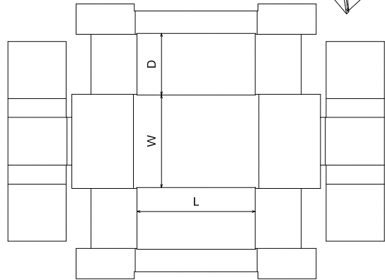
FEFCO\0400 - Folder Type Boxes\FEFCO 0433
