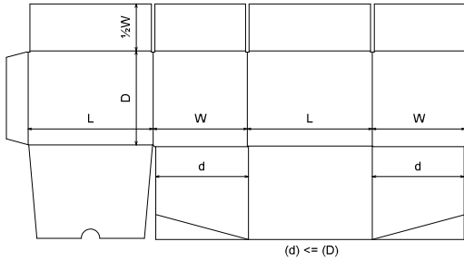
FEFCO\0200 - Slotted Type Boxes\FEFCO 0225 - Regular Slotted Top, File Base
