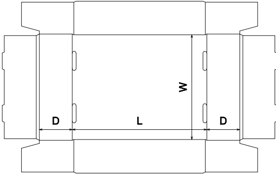
FEFCO\0400 - Folder Type Boxes\FEFCO 0422
