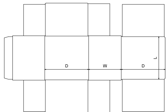
FEFCO\0400 - Folder Type Boxes\FEFCO 0443
