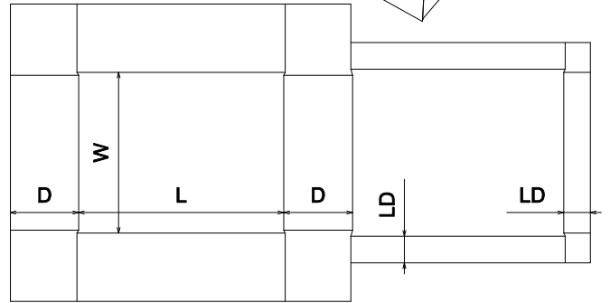
FEFCO\0400 - Folder Type Boxes\FEFCO 0441
