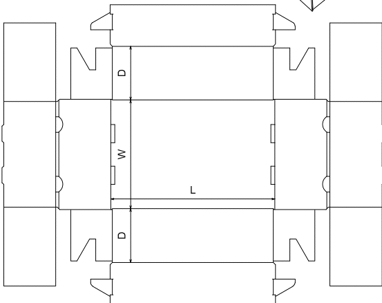
FEFCO\0400 - Folder Type Boxes\FEFCO 0432
