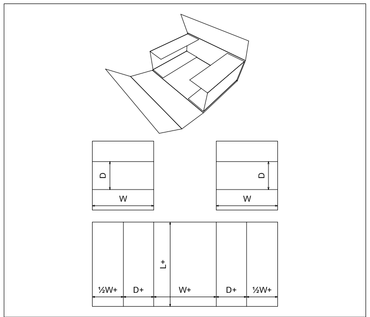
FEFCO\0400 - Folder Type Boxes\FEFCO 0405
