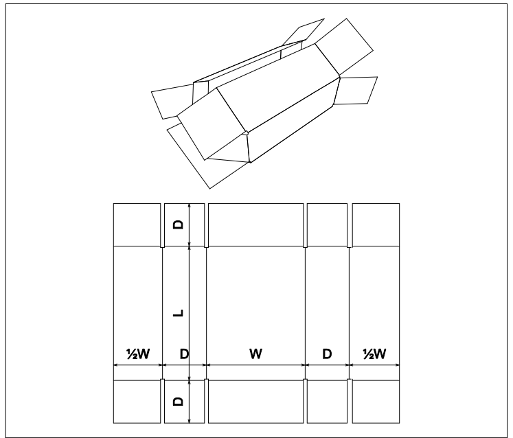
FEFCO\0400 - Folder Type Boxes\FEFCO 0411
