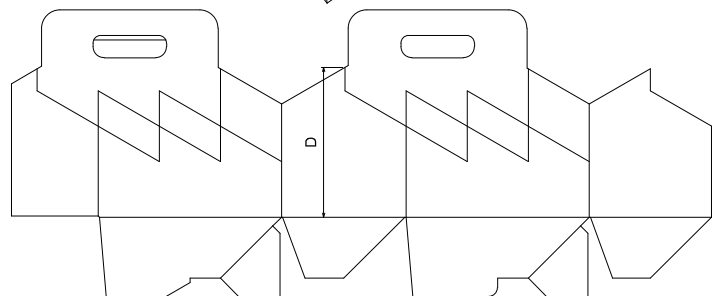
FEFCO\0700 - Ready Glued Cases\FEFCO 0717 - Bottle Carrier
