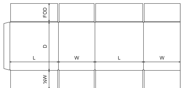
FEFCO\0200 - Slotted Type Boxes\FEFCO 0214 - Roll Over Top Slotted Container
