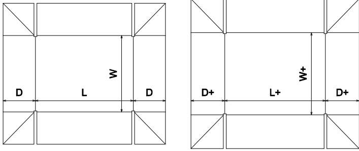
FEFCO\0300 - Telescope Type Box\FEFCO 0308
