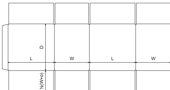
FEFCO\0200 - Slotted Type Boxes\FEFCO 0202 - Overlapping Slotted Container
