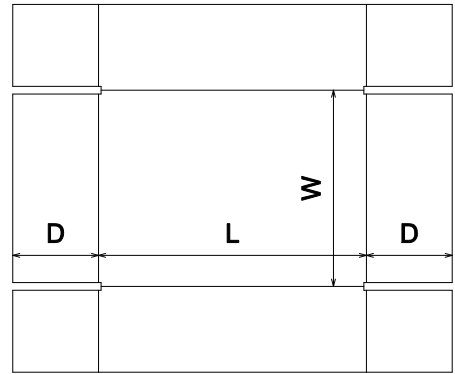
FEFCO\0400 - Folder Type Boxes\FEFCO 0453
