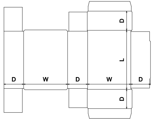
FEFCO\0400 - Folder Type Boxes\FEFCO 0447
