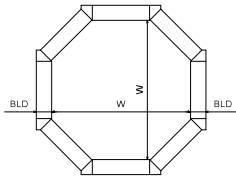
FEFCO\0300 - Telescope Type Box\FEFCO 0350
