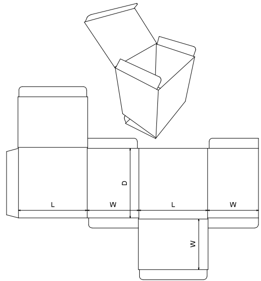
FEFCO\0200 - Slotted Type Boxes\FEFCO 0211 - Tuck to Front Top, Tuck to Back Base
