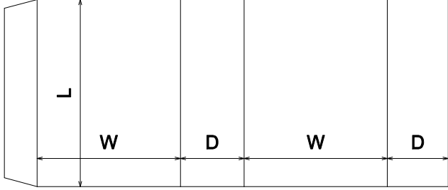
FEFCO\0500 - Slide Type Boxes\FEFCO 0503
