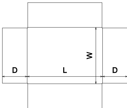
FEFCO\0400 - Folder Type Boxes\FEFCO 0458
