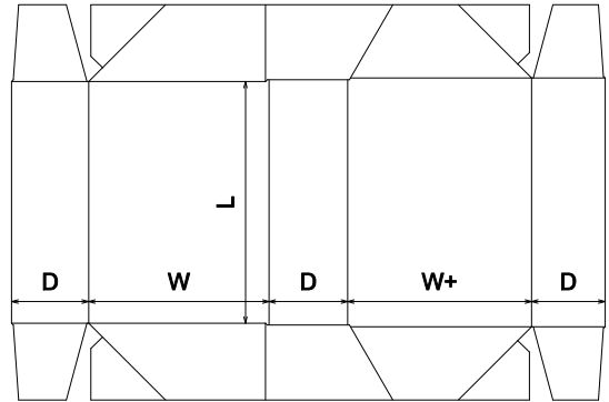
FEFCO\0700 - Ready Glued Cases\FEFCO 0759
