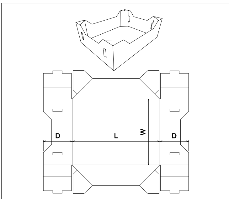
FEFCO\0700 - Ready Glued Cases\FEFCO 0771
