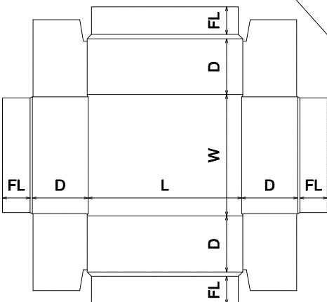
FEFCO\0400 - Folder Type Boxes\FEFCO 0430
