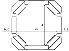
FEFCO\0300 - Telescope Type Box\FEFCO 0351
