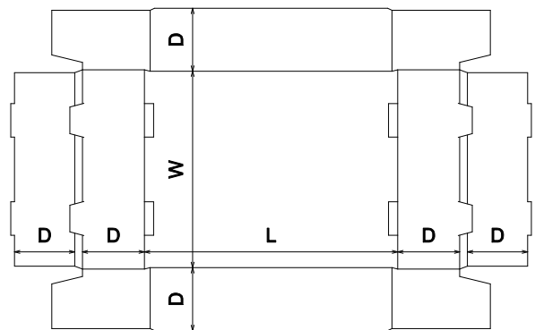
FEFCO\0400 - Folder Type Boxes\FEFCO 0435
