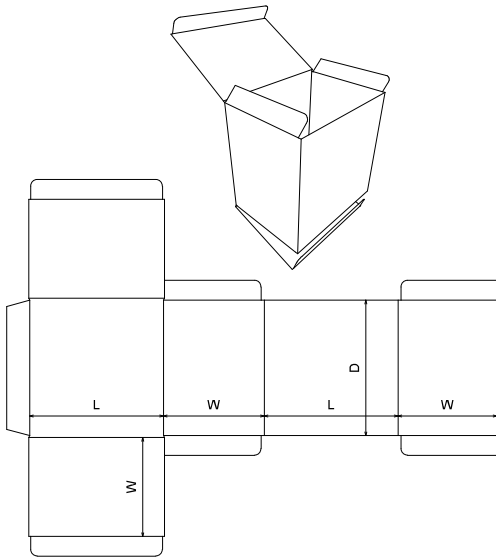
FEFCO\0200 - Slotted Type Boxes\FEFCO 0210 - Tuck to Front Container
