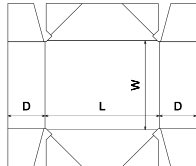
FEFCO\0400 - Folder Type Boxes\FEFCO 0451
