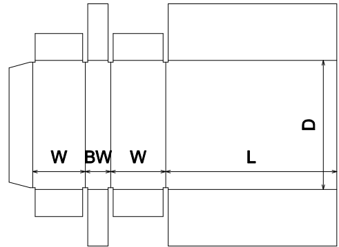
FEFCO\0600 - Rigid Type Boxes\FEFCO 0621
