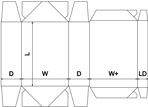
FEFCO\0700 - Ready Glued Cases\FEFCO 0761
