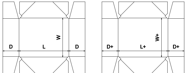
FEFCO\0300 - Telescope Type Box\FEFCO 0304
