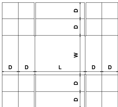
FEFCO\0400 - Folder Type Boxes\FEFCO 0456
