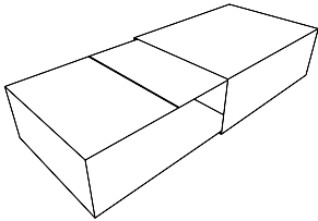
FEFCO\0500 - Slide Type Boxes\FEFCO 0511
