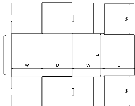
FEFCO\0400 - Folder Type Boxes\FEFCO 0470
