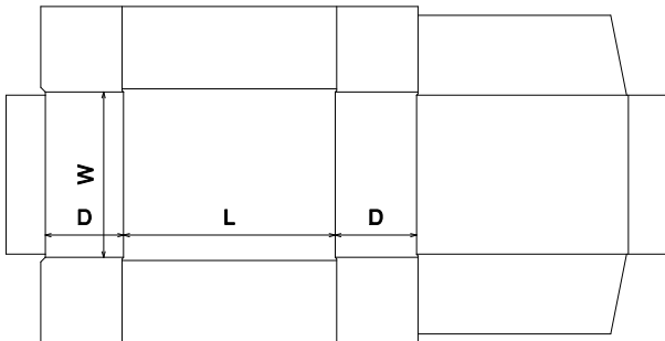
FEFCO\0400 - Folder Type Boxes\FEFCO 0440
