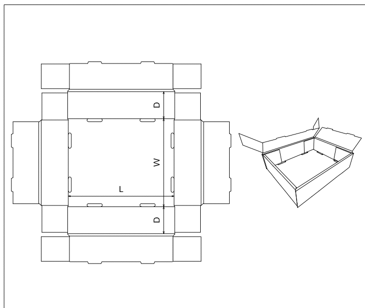
FEFCO\0400 - Folder Type Boxes\FEFCO 0425
