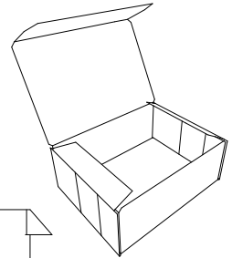
FEFCO\0400 - Folder Type Boxes\FEFCO 0447
