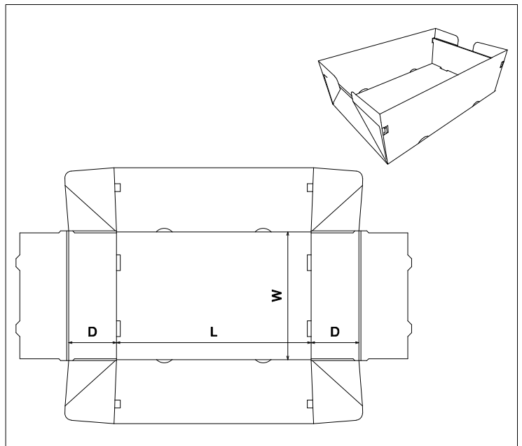
FEFCO\0700 - Ready Glued Cases\FEFCO 0772
