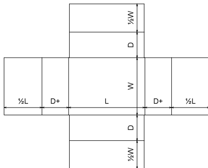
FEFCO\0400 - Folder Type Boxes\FEFCO 0402
