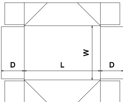
FEFCO\0400 - Folder Type Boxes\FEFCO 0450
