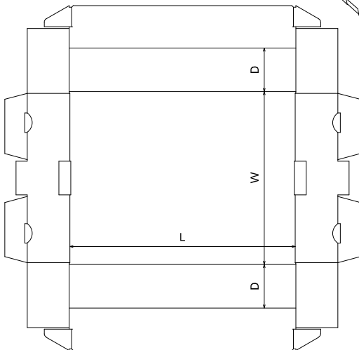
FEFCO\0400 - Folder Type Boxes\FEFCO 0436
