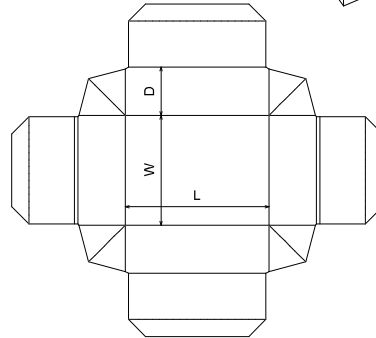
FEFCO\0300 - Telescope Type Box\FEFCO 0323
