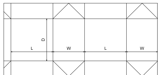
FEFCO\0200 - Slotted Type Boxes\FEFCO 0226 - Gusset Style Container
