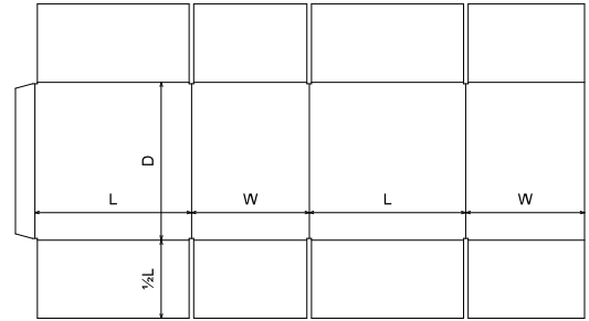
FEFCO\0200 - Slotted Type Boxes\FEFCO 0205 - Width Panels Meet, Slotted Container
