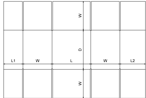
FEFCO\0200 - Slotted Type Boxes\FEFCO 0230
