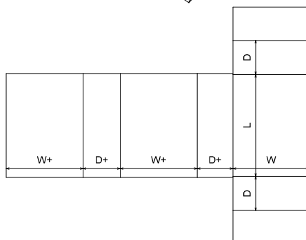
FEFCO\0400 - Folder Type Boxes\FEFCO 0400
