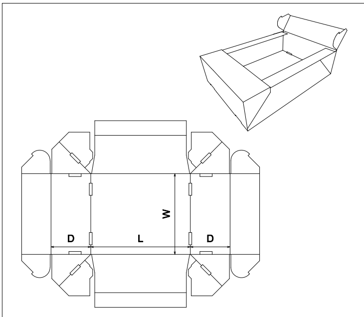
FEFCO\0700 - Ready Glued Cases\FEFCO 0773
