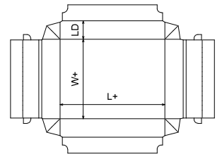
FEFCO\0300 - Telescope Type Box\FEFCO 0323
