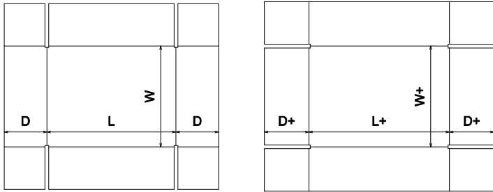
FEFCO\0300 - Telescope Type Box\FEFCO 0301
