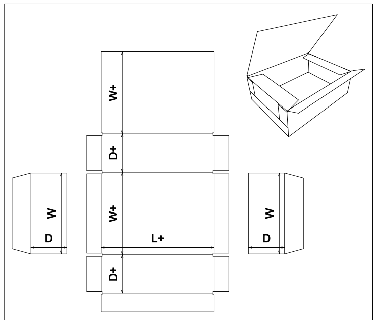
FEFCO\0600 - Rigid Type Boxes\FEFCO 0601
