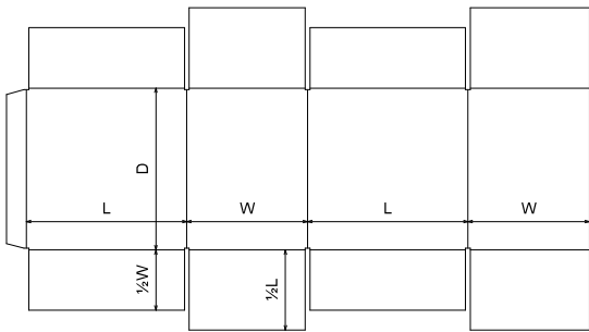
FEFCO\0200 - Slotted Type Boxes\FEFCO 0204 - All Flaps Meet Slotted Container
