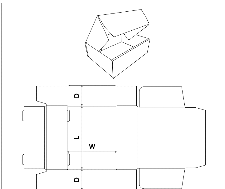
FEFCO\0400 - Folder Type Boxes\FEFCO 0426
