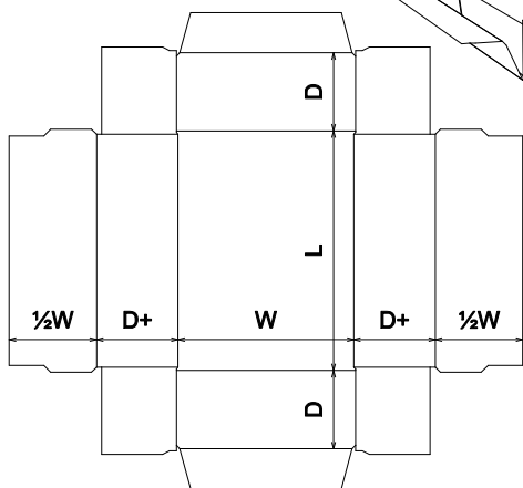
FEFCO\0400 - Folder Type Boxes\FEFCO 0415
