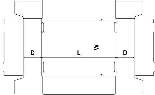
FEFCO\0400 - Folder Type Boxes\FEFCO 0421
