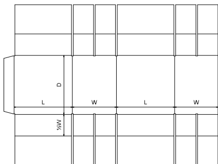
FEFCO\0200 - Slotted Type Boxes\FEFCO 0208 - Slotted Containers with Holders
