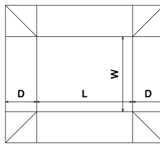
FEFCO\0300 - Telescope Type Box\FEFCO 0309
