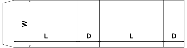
FEFCO\0500 - Slide Type Boxes\FEFCO 0502
