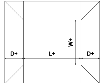
FEFCO\0300 - Telescope Type Box\FEFCO 0309
