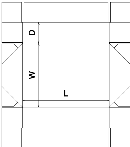
FEFCO\0700 - Ready Glued Cases\FEFCO 0718
