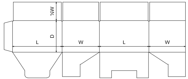
FEFCO\0200 - Slotted Type Boxes\FEFCO 0216 - Regular Slotted Top, Envelope Base
