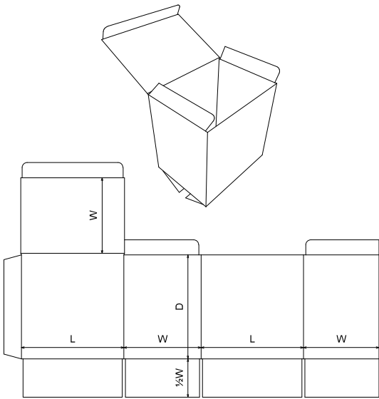
FEFCO\0200 - Slotted Type Boxes\FEFCO 0212 - Tuck to Front Top, Regular Slotted Base
