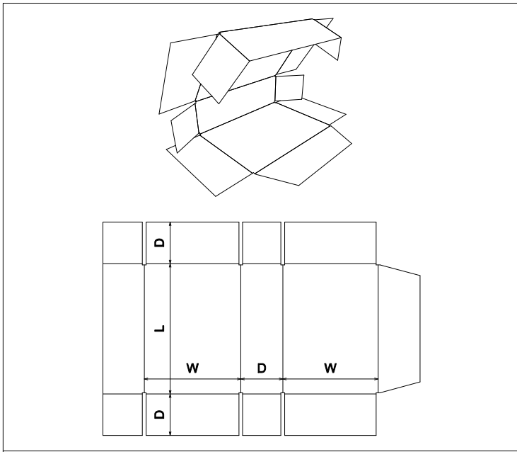
FEFCO\0400 - Folder Type Boxes\FEFCO 0410
