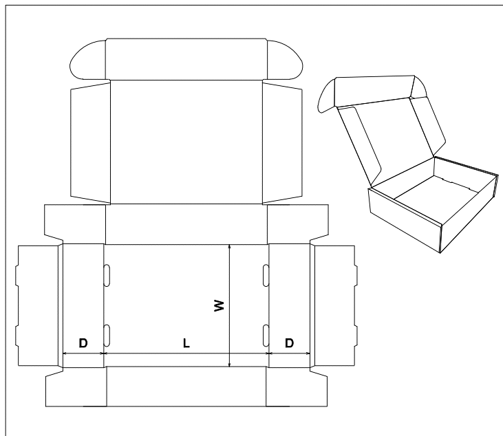
FEFCO\0400 - Folder Type Boxes\FEFCO 0427
