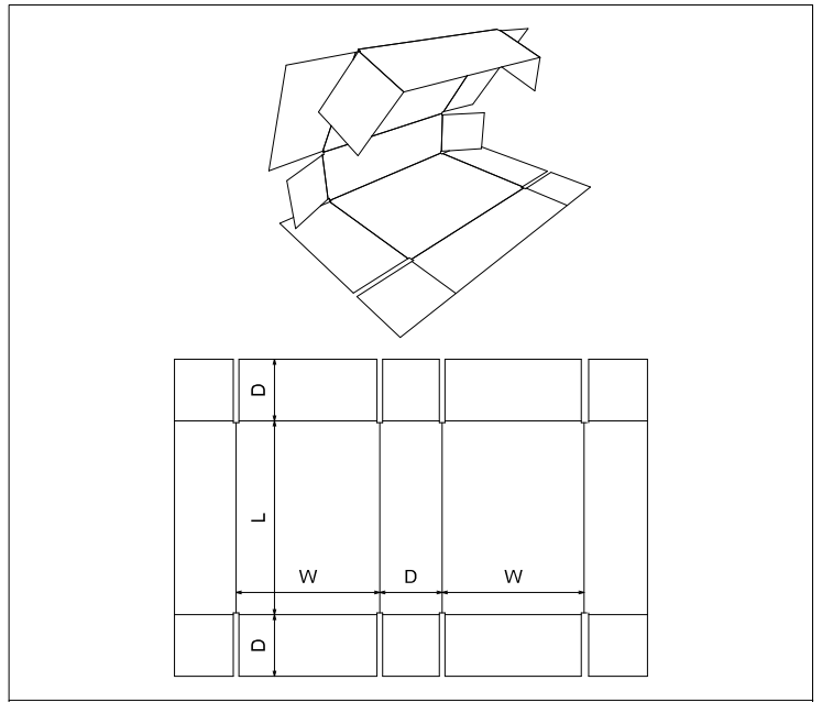
FEFCO\0400 - Folder Type Boxes\FEFCO 0409
