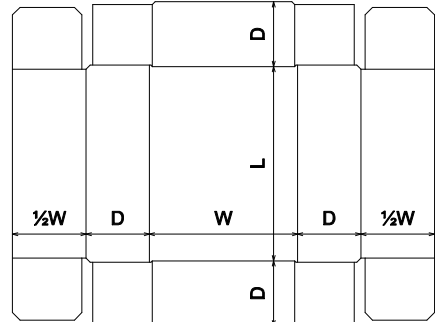
FEFCO\0400 - Folder Type Boxes\FEFCO 0416
