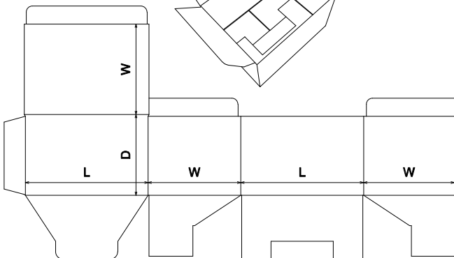
FEFCO\0200 - Slotted Type Boxes\FEFCO 0215 - Tuck to Front Top, Envelope Base
