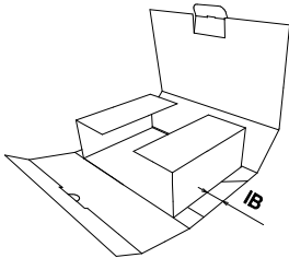
FEFCO\0300 - Telescope Type Box\FEFCO 0301
