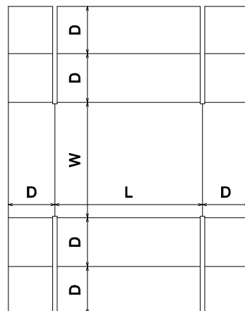
FEFCO\0400 - Folder Type Boxes\FEFCO 0455
