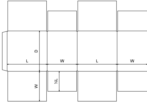
FEFCO\0200 - Slotted Type Boxes\FEFCO 0206 - Length Panels Overlap, Width Panels Meet
