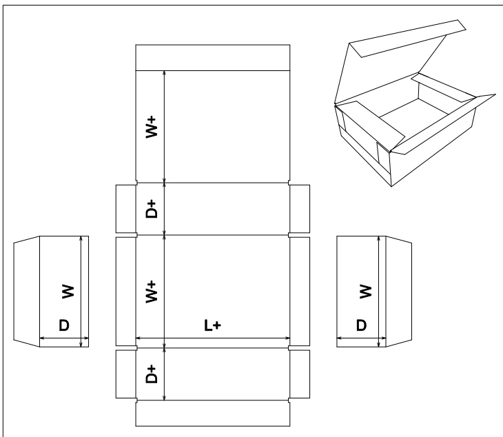
FEFCO\0600 - Rigid Type Boxes\FEFCO 0602
