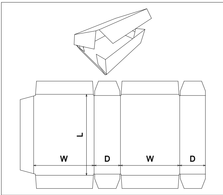
FEFCO\0400 - Folder Type Boxes\FEFCO 0406
