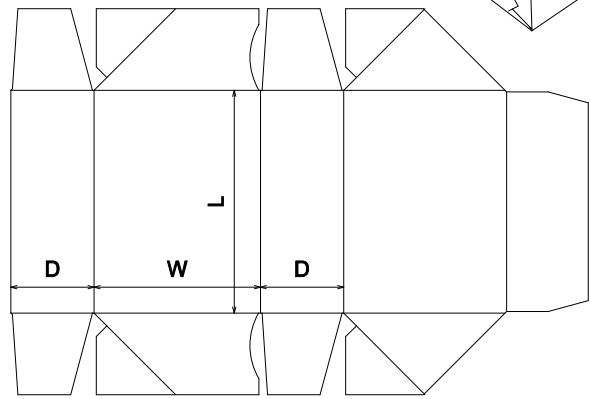
FEFCO\0700 - Ready Glued Cases\FEFCO 0751
