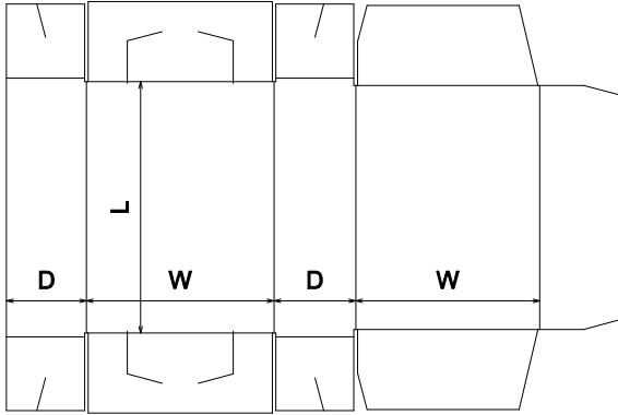
FEFCO\0400 - Folder Type Boxes\FEFCO 0442
