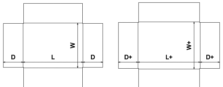
FEFCO\0300 - Telescope Type Box\FEFCO 0302
