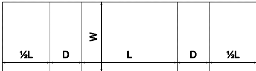
FEFCO\0500 - Slide Type Boxes\FEFCO 0509
