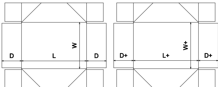
FEFCO\0300 - Telescope Type Box\FEFCO 0303
