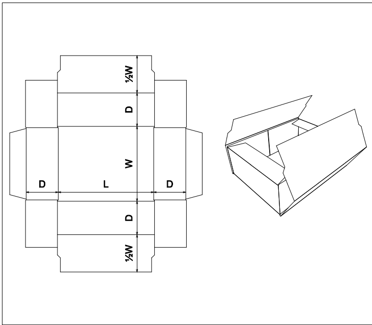
FEFCO\0400 - Folder Type Boxes\FEFCO 0412
