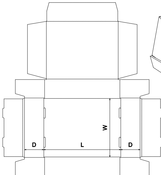
FEFCO\0400 - Folder Type Boxes\FEFCO 0429
