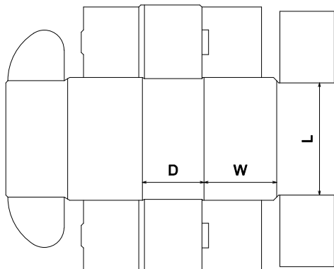
FEFCO\0400 - Folder Type Boxes\FEFCO 0471
