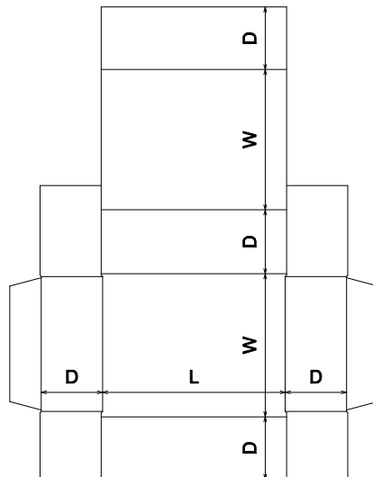
FEFCO\0400 - Folder Type Boxes\FEFCO 0413
