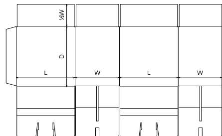
FEFCO\0200 - Slotted Type Boxes\FEFCO 0207 - Slotted Container with Dividers
