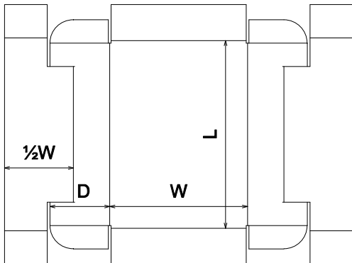
FEFCO\0400 - Folder Type Boxes\FEFCO 0446
