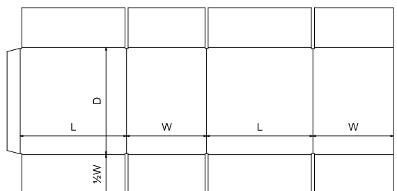
FEFCO\0200 - Slotted Type Boxes\FEFCO 0201 - Regular Slotted Container
