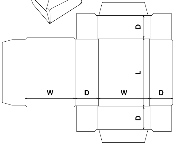
FEFCO\0400 - Folder Type Boxes\FEFCO 0420
