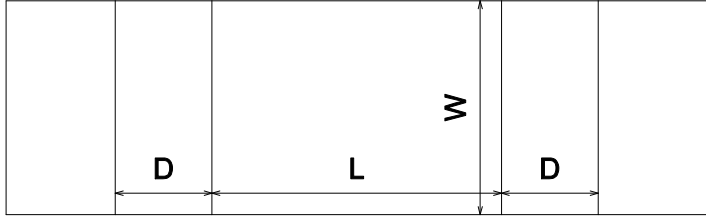
FEFCO\0900 - Interior Fitments\FEFCO 0907
