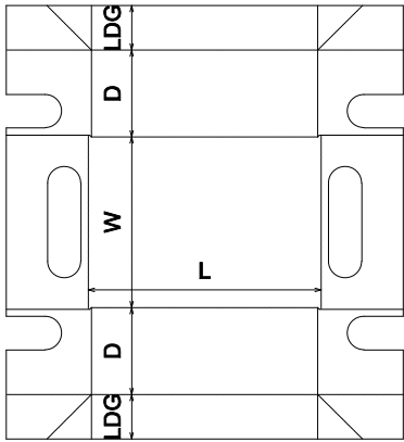
FEFCO\0400 - Folder Type Boxes\FEFCO 0434
