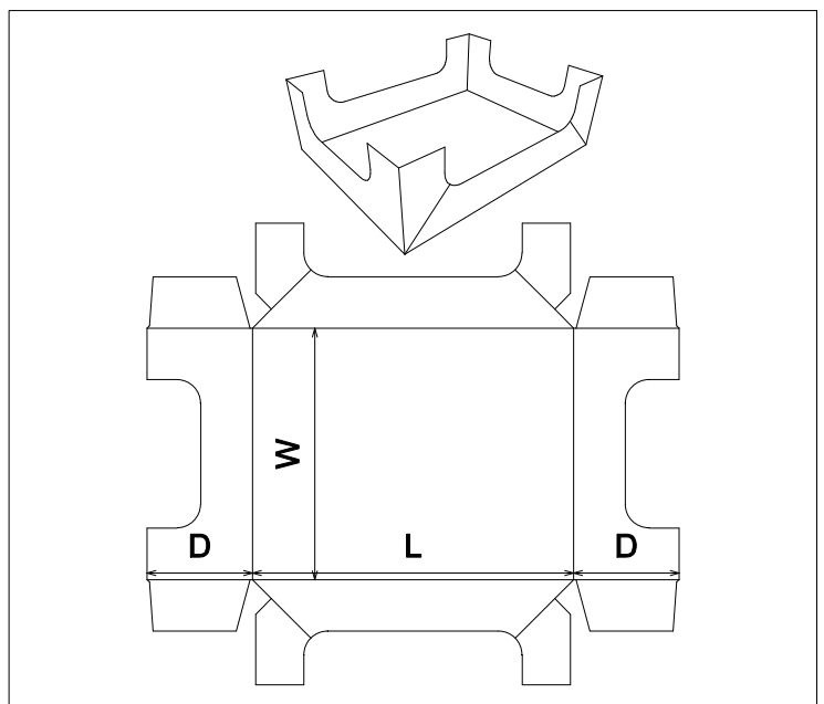
FEFCO\0700 - Ready Glued Cases\FEFCO 0770
