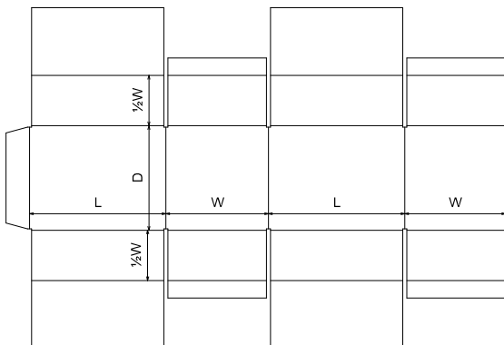
FEFCO\0200 - Slotted Type Boxes\FEFCO 0229
