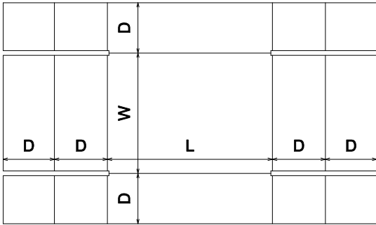
FEFCO\0400 - Folder Type Boxes\FEFCO 0454
