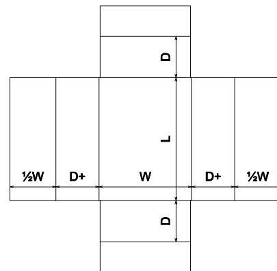
FEFCO\0400 - Folder Type Boxes\FEFCO 0401
