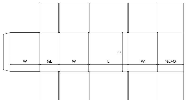
FEFCO\0200 - Slotted Type Boxes\FEFCO 0228
