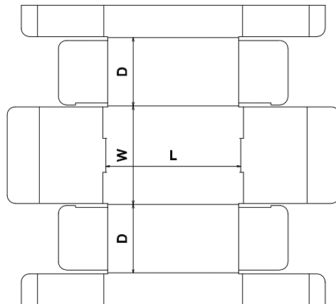
FEFCO\0400 - Folder Type Boxes\FEFCO 0431
