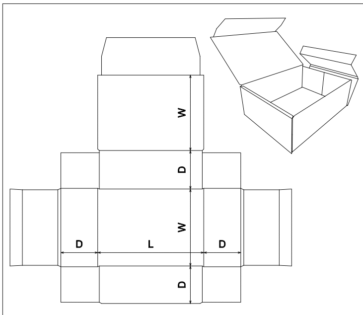
FEFCO\0400 - Folder Type Boxes\FEFCO 0428
