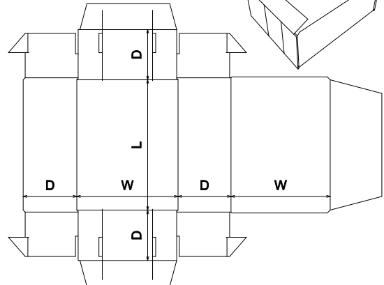
FEFCO\0400 - Folder Type Boxes\FEFCO 0445
