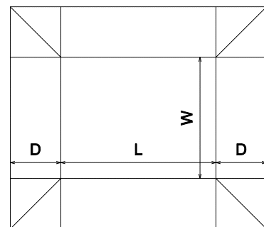
FEFCO\0400 - Folder Type Boxes\FEFCO 0449
