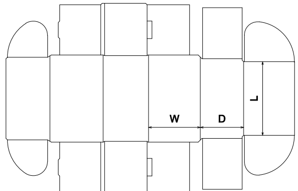
FEFCO\0400 - Folder Type Boxes\FEFCO 0472
