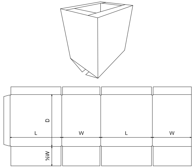
FEFCO\0200 - Slotted Type Boxes\FEFCO 0209 - Flange Top, Regular Slotted Base
