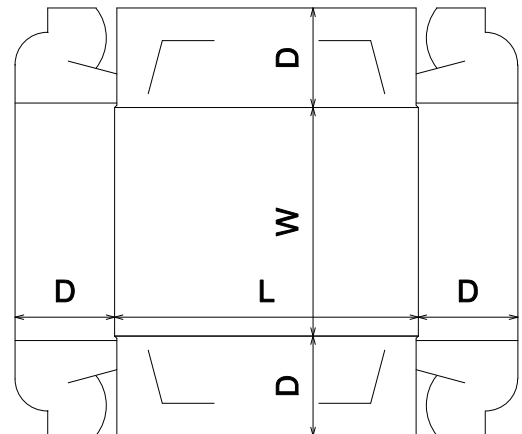
FEFCO\0400 - Folder Type Boxes\FEFCO 0457
