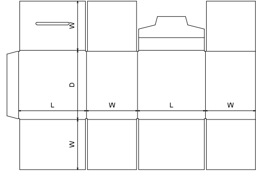
FEFCO\0200 - Slotted Type Boxes\FEFCO 0218
