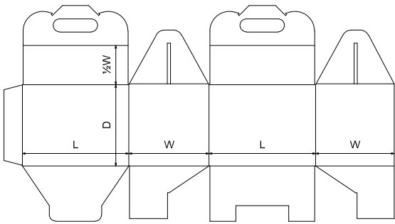
FEFCO\0200 - Slotted Type Boxes\FEFCO 0217 - Carry Handle Top, Envelope Base
