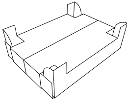
FEFCO\0400 - Folder Type Boxes\FEFCO 0448
