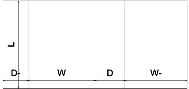
FEFCO\0900 - Interior Fitments\FEFCO 0906
